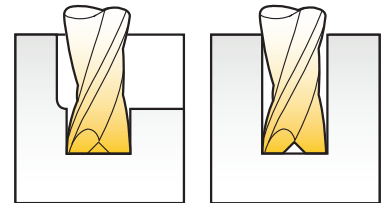
Slotting Engraving
