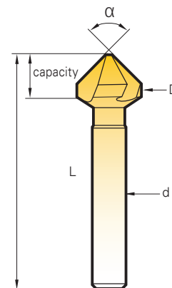
Countersink
